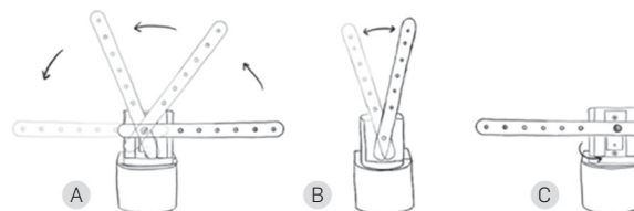
Figure 5. (A) The timer motion moves 30 positions right to left and then 30 positions left to right, advancing 6 degrees per step, (B) The wave motion waves back and forth 6 times, and (C) the reset sequence centers and lowers the arm.
