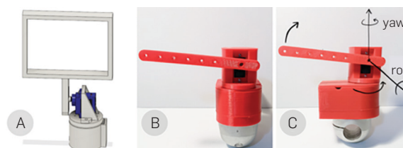
Figure 4. (A) Early prototype 3D model, (B) front view, and (C) side view of fabricated sidekick with wheelchair mount.
