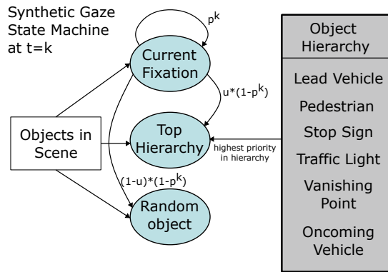
Fig. 4: Synthetic gaze generated by a state machine, shown at time t = k : after a transition to a new object, it becomes the current fixation. The process repeats at every timestep.
