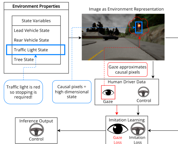
Fig. 1: Outline of training for imitation learning with gaze as a supervisory signal for approximating causal information in the scene. Here gaze pixels represent a noisy approximation of the causal pixels in the RGB image space, while the causal pixels are an abstraction of the causal scene elements. Gaze is only required at train time.
