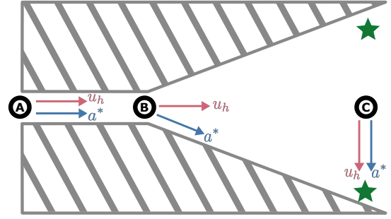
Fig. 2: Diagram of user input ( u ) and optimal robot motion ( a^* ) during an example task. The user moves a point robot to one of the green stars. At A , user input and optimal motion are both to the right. At B , user input is still directly to the right, but the optimal motion is diagonally towards the goal. At C , both the user input and the optimal motion point towards the goal. Early prediction improves task performance only at B .
