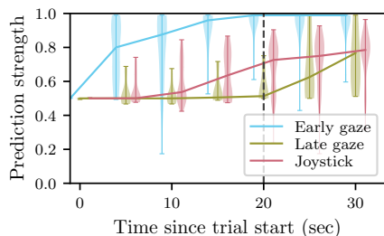
Fig. 7: Distributions of prediction strength over all trials for early gaze, late gaze, and joystick. The x -axis here is not normalized by trial time. The dashed line at 20s indicates the cutoff time T_c for early gaze prediction.
